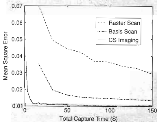
[FIG4] Average MSE for RS, BS, and CS single-pixel images as a function of the total image capture time T (real data).
