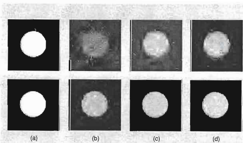
[FIG3] Frame 32 from a reconstructed video sequence using (top row) M = 20,000 and (bottom row) M = 50,000 measurements (simulation from [10]). (a) Original frame of an N = 64 \times 64 \times 64 video of a disk simultaneously dilating and translating. (b) Frame-by-frame 2-D measurements + frame-by-frame 2-D reconstruction; MSE = 3.63 and 0.82, respectively. (c) Frame-by-frame 2-D measurements + joint 3-D reconstruction; MSE = 0.99 and 0.24, respectively. (d) Joint 3-D measurements + joint 3-D reconstruction; MSE = 0.76 and 0.18, respectively.
